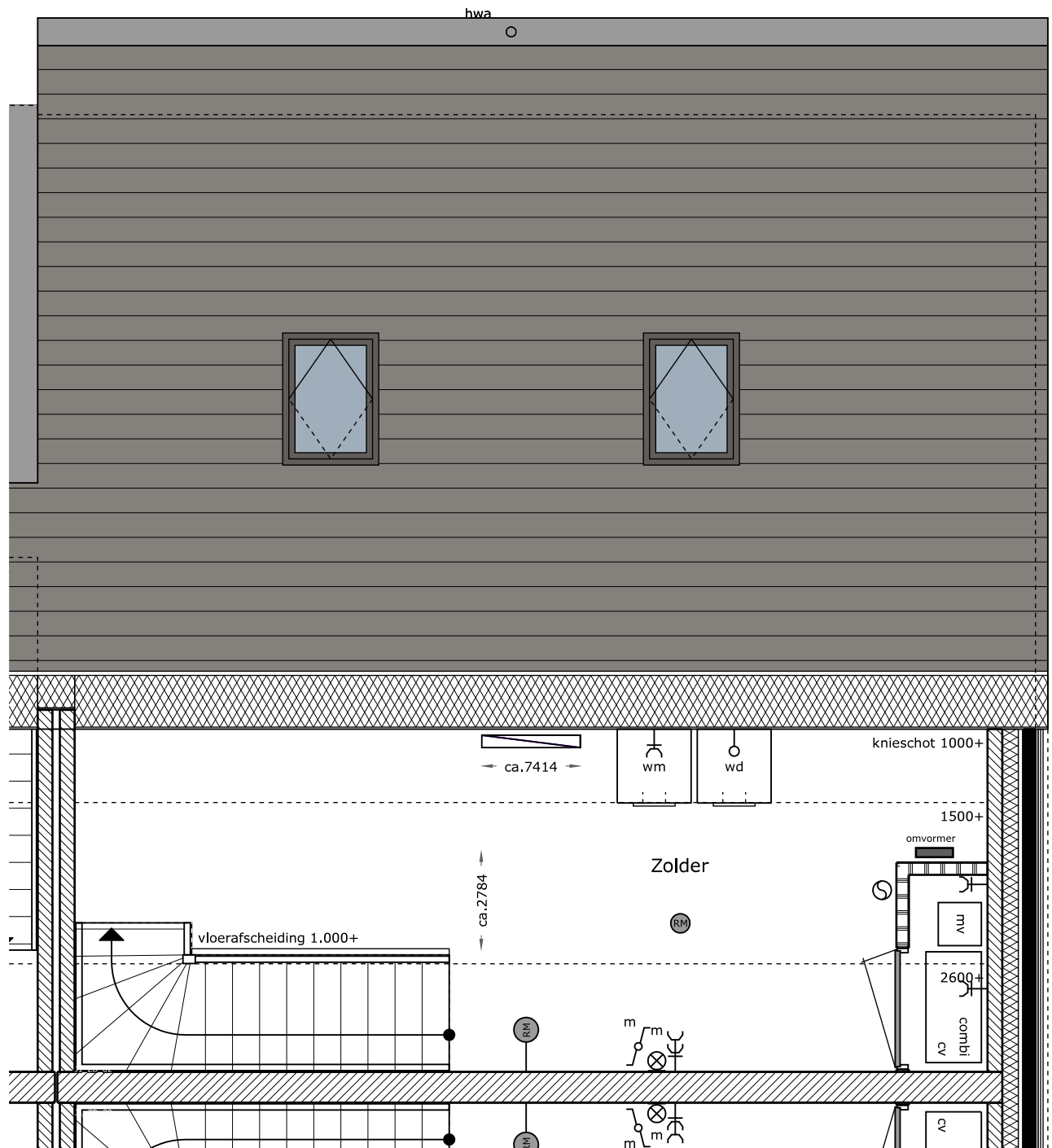
Zolder
