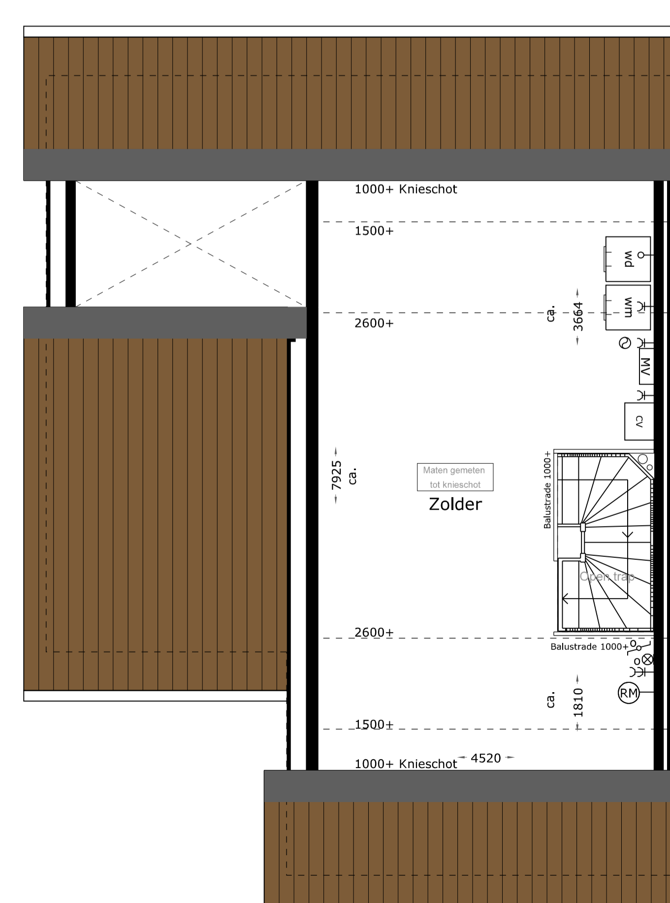
Zolder
